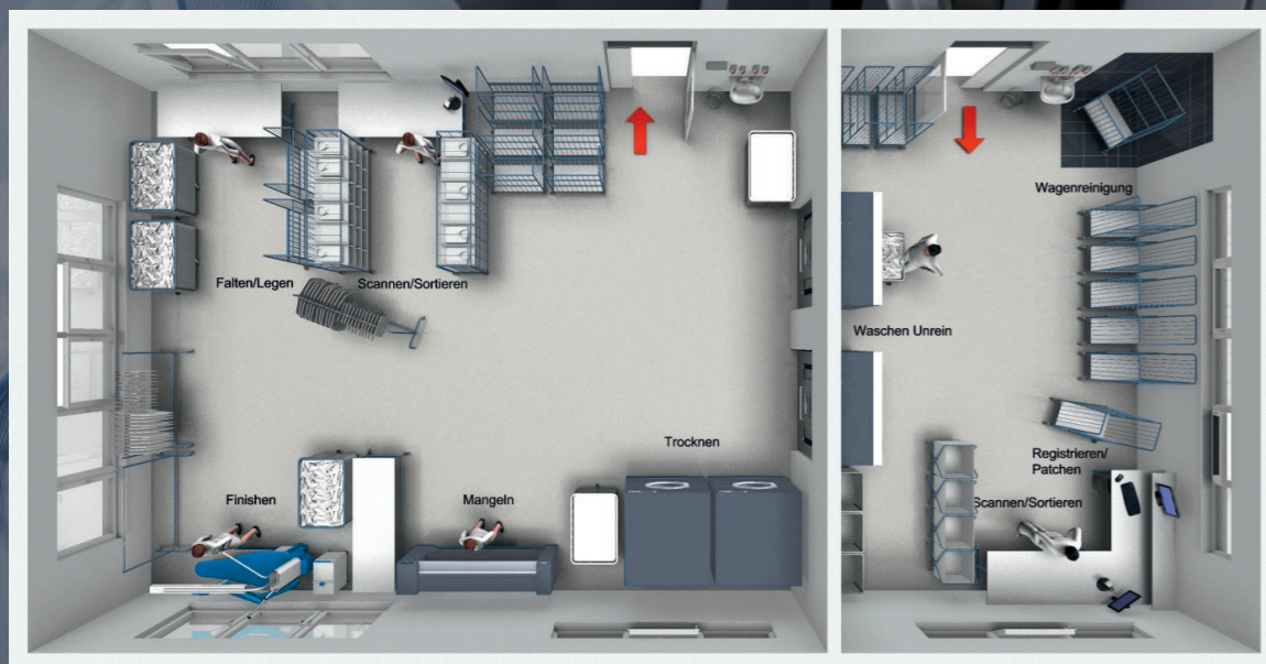
A typical room layout for a barrier wash system with clean and dirty sides
